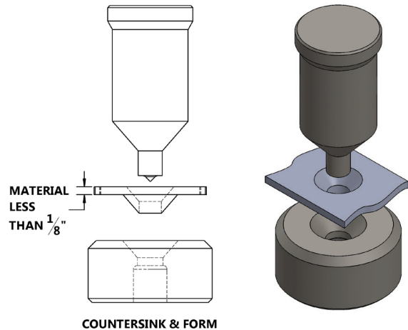
COUNTERSINK & FORM
